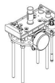
VIBRATORY HOLDER
